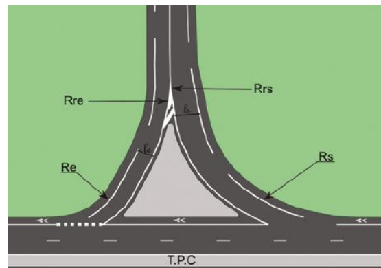
Figure 57 : Demi-carrefour (Source : Cerema)
